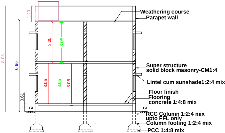
SECTION ELEVATION
