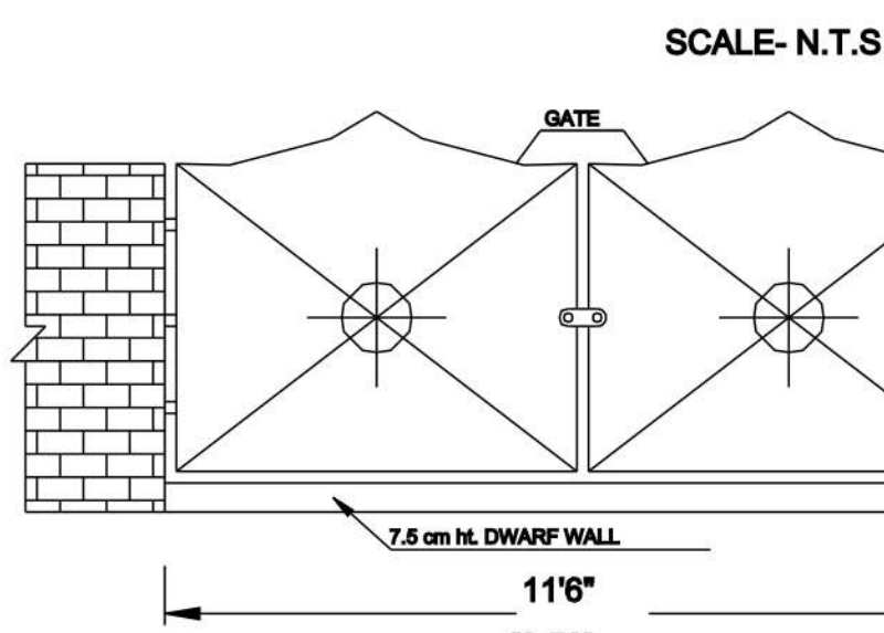
GATE AND COMPOUND WALL DETAILS
