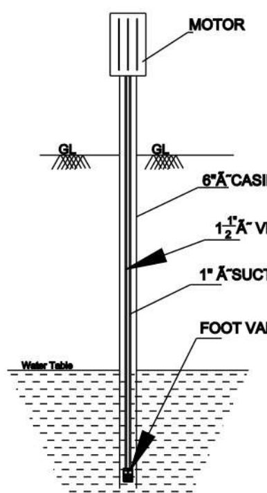
SEC. OF BOREWELL
