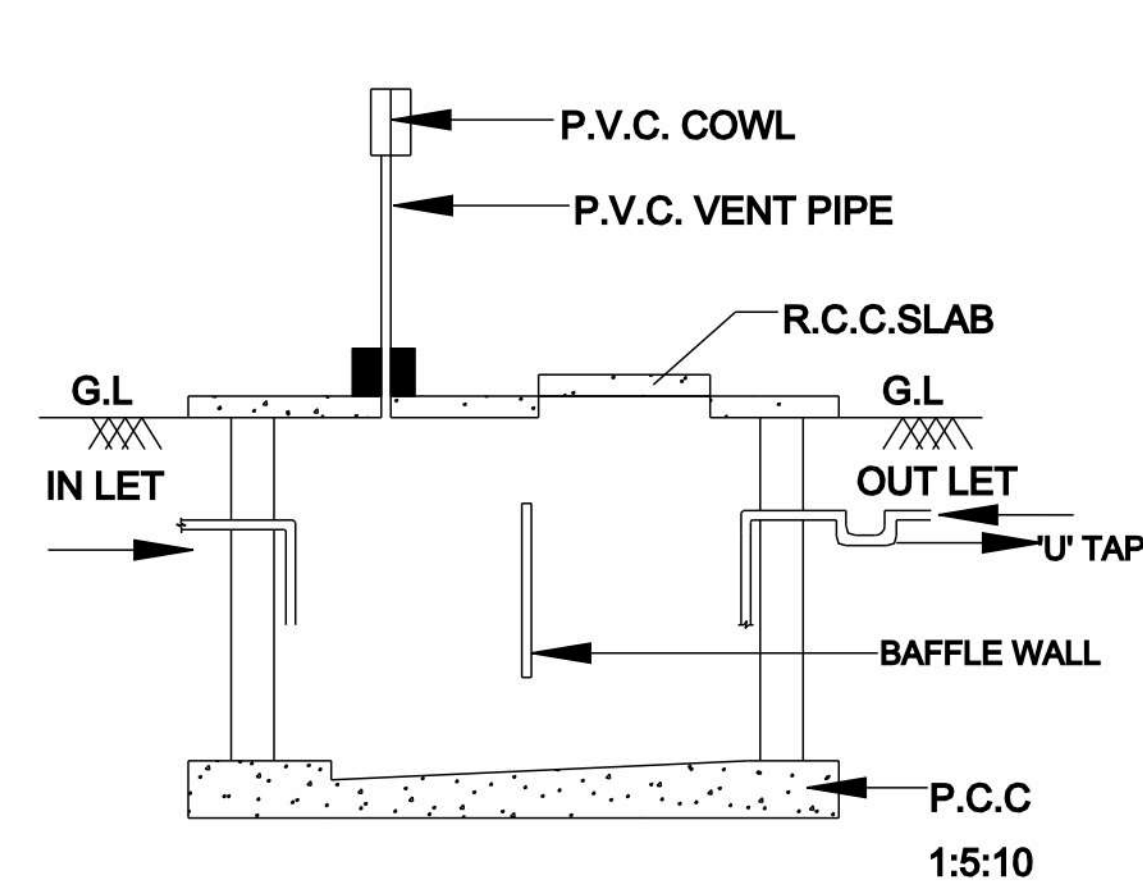
SEC. OF SEPTIC TANK
