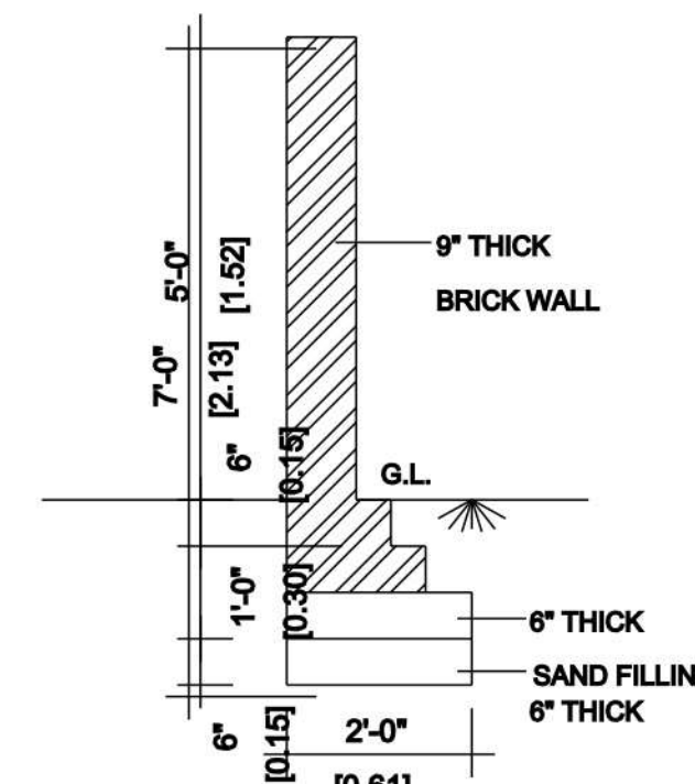
SECTION OF COMPOUND WALL
