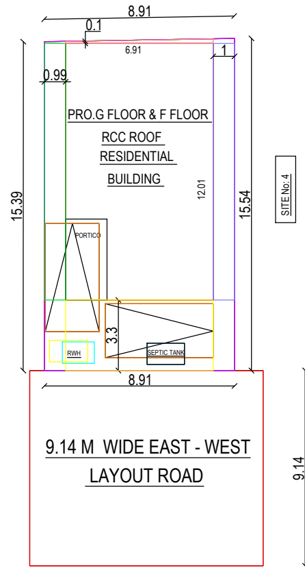
SITE PLAN
