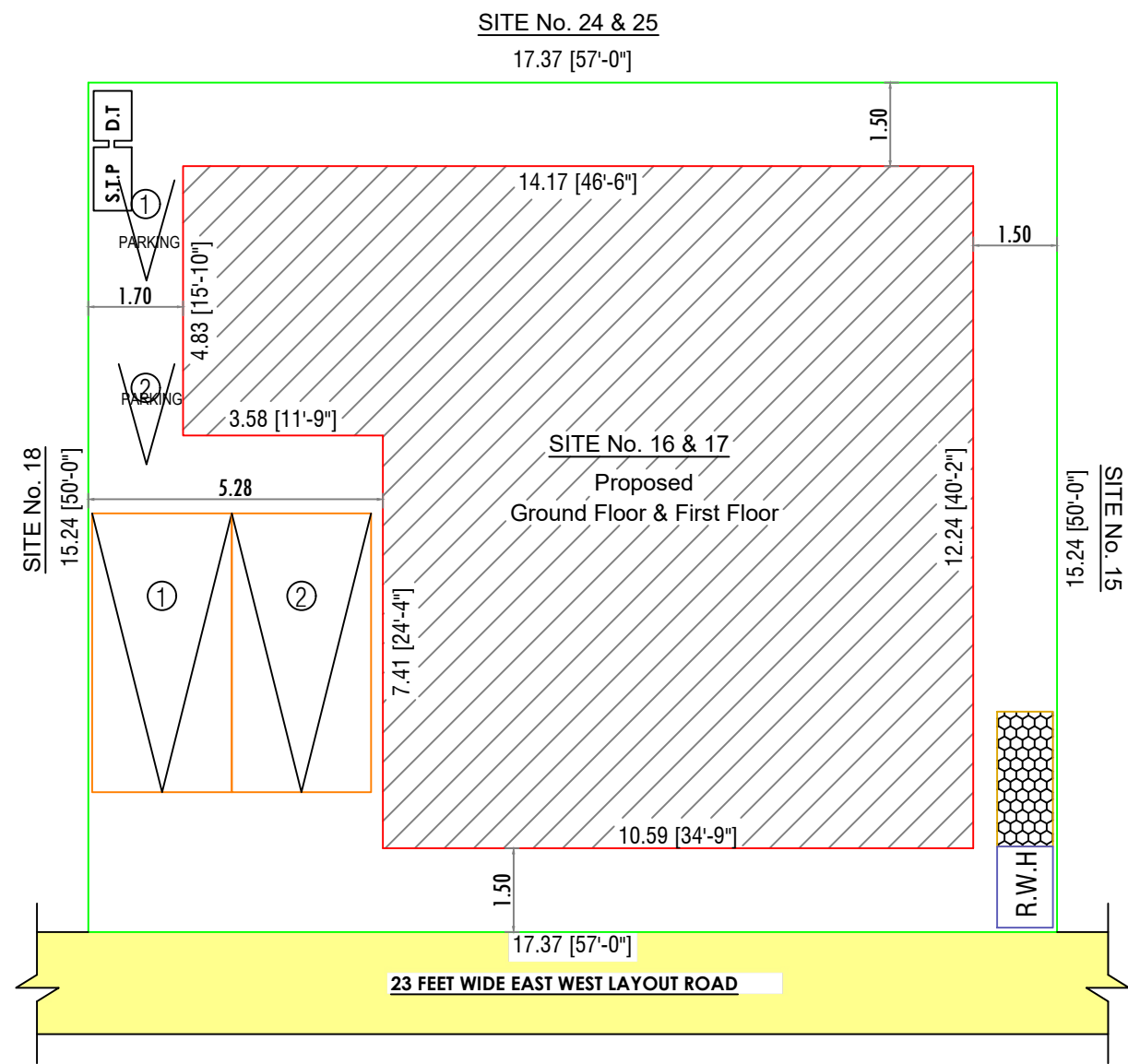
SITE PLAN
