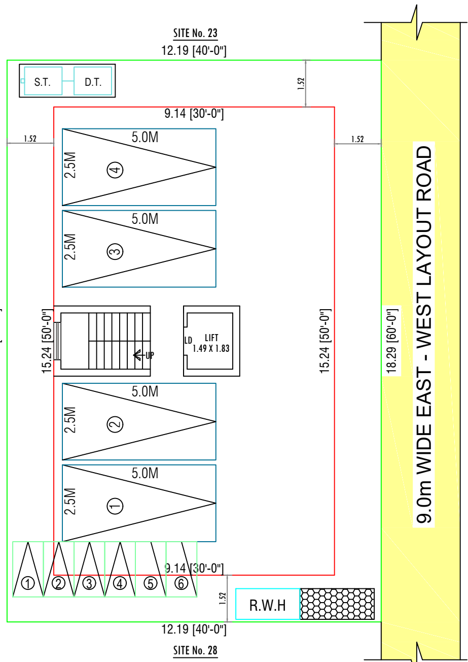
SITE PLAN
