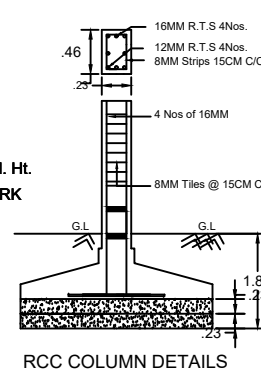
RCC COLUMN DETAILS
