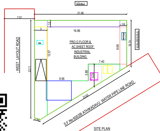
SITE PLAN
