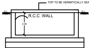
RWHP SECTION (SAMPLE) RWHP_CAPACITY_L = 2000LTRS
