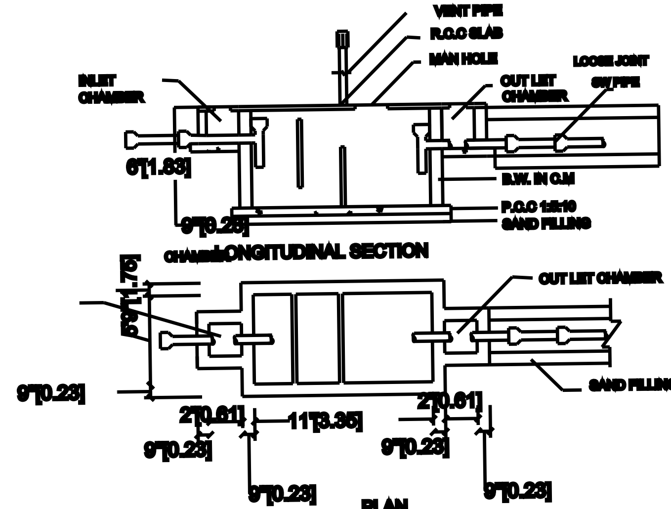
SEPTIC TANK:
