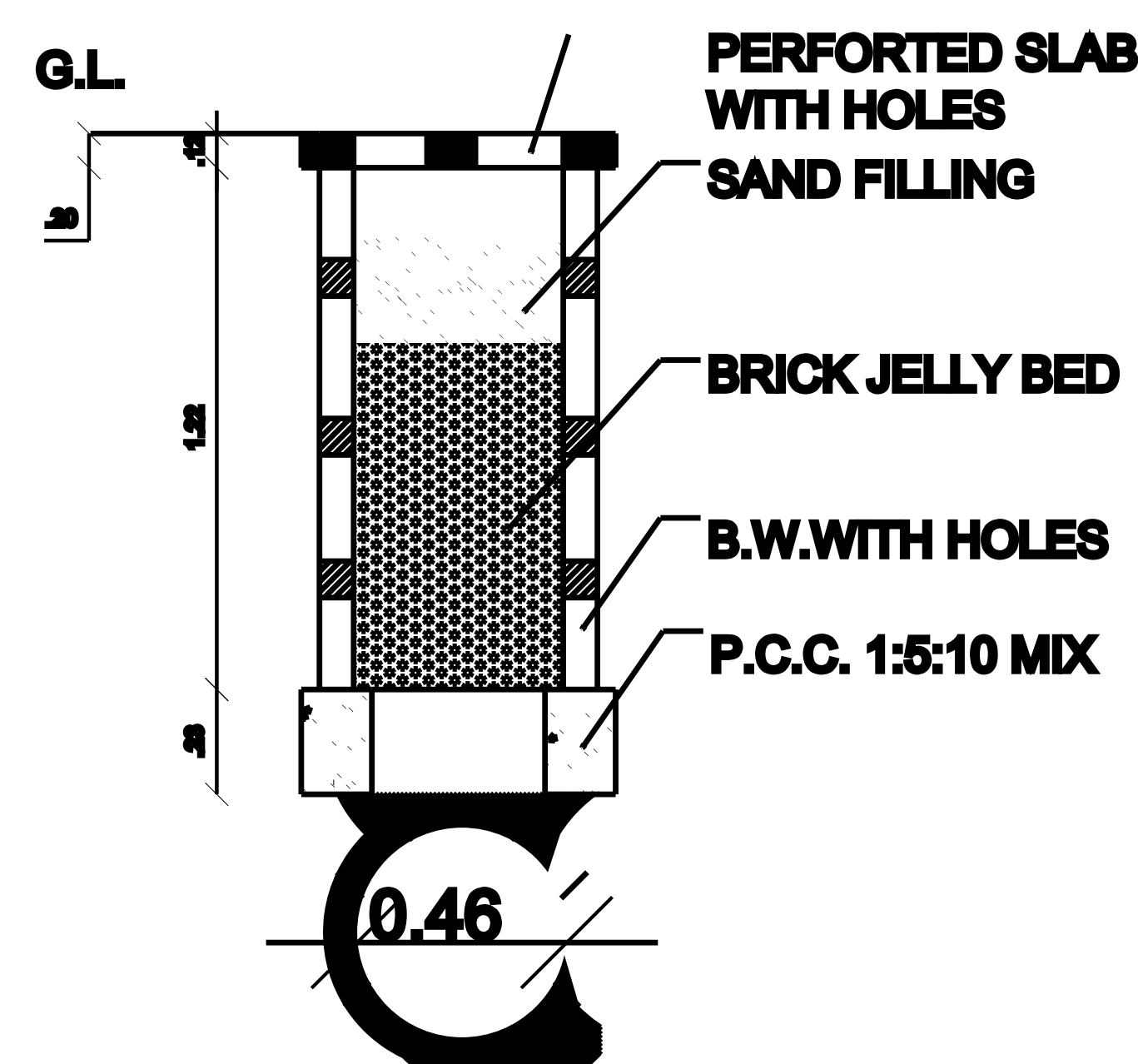
RAIN WATER HARVEST
