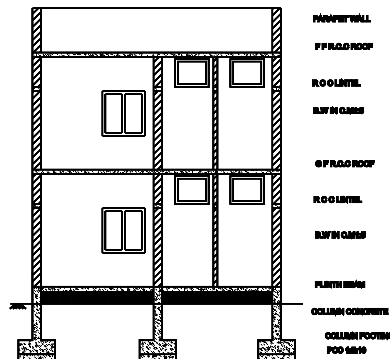
SECTION-AA
