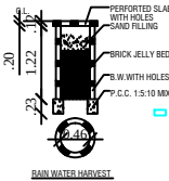
RAIN WATER HARVEST
