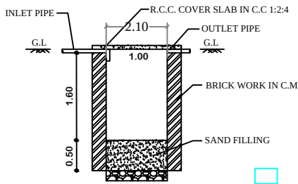
SECTIONAL DETAILS
