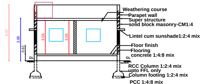
SECTION ELEVATION
