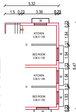
POSED FIRST OR PLAN
