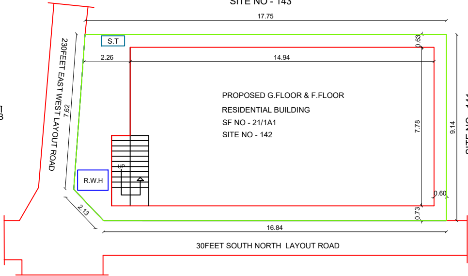
SITE PLAN
