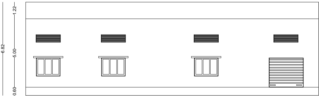
SOUTH ELEVATION
