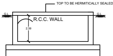
RWH SECTION (SAMPLE) RWH_CAPACITY_L = 2000LTRS
