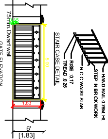
STAIR CASE DETAIL
