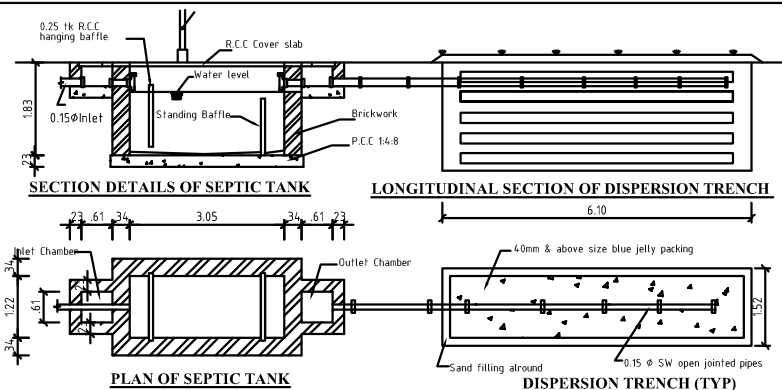
DETAILS OF SEPTIC TANK - 250 GALLONS & DISPERSION TRENCH
