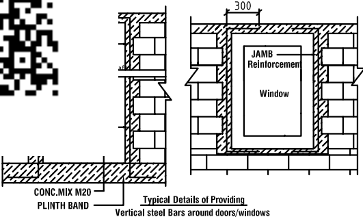
Essential Internal Elements in Buildings for Earthquake safety
