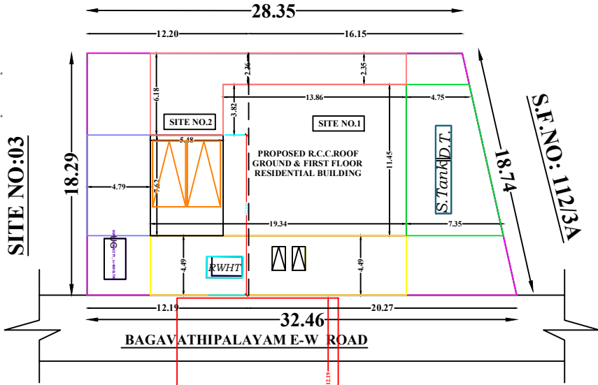
SITE PLAN
