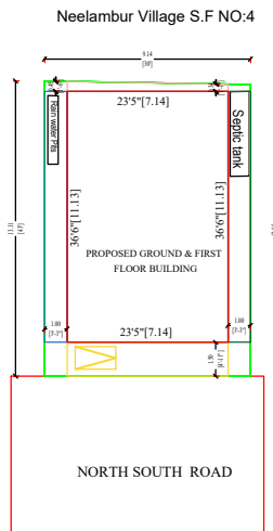
SITE PLAN
