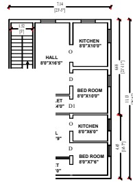
IRST FLOOR PLAN
