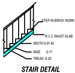
STAIR DETAIL
