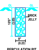
PERCOLATION PIT
