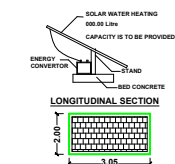
SOLAR SYSTEM
