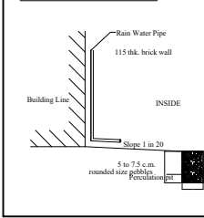
PERCOLATION PIT
