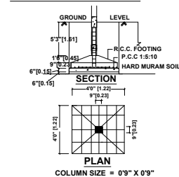
FOUNDATION DETAILS
