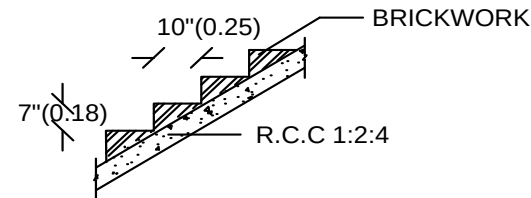
STAIRCASE WAIST SLAB
