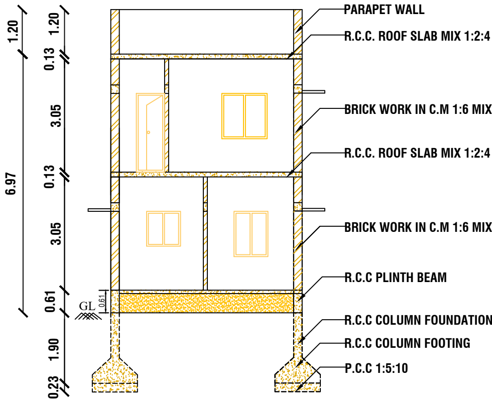
CROSS SECTION AT A-A
