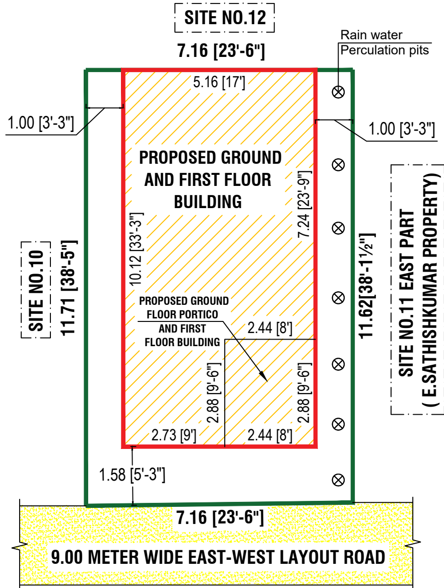
SITE PLAN
