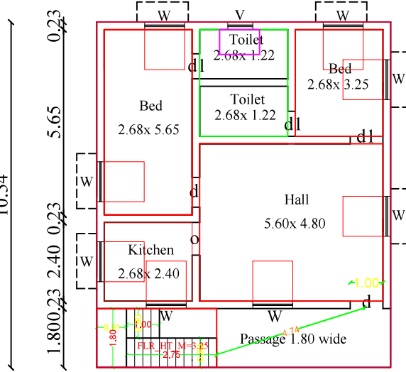
PLAN for Proposed First Floor
