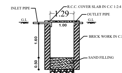
SECTIONAL DETAILS
