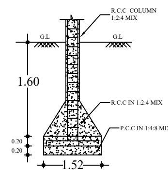
R.C.C. COLUMN DETAILS
