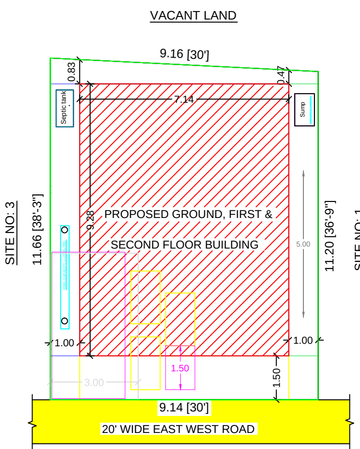
SITE PLAN
