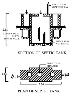
SEPTIC TANK
