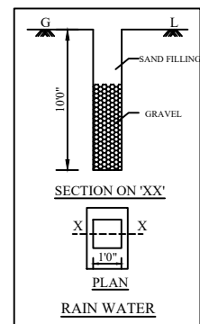
RAINWATER HARVESTING
