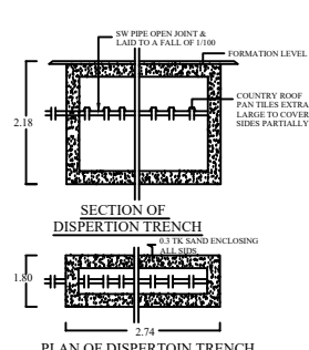
DISPERSION TRENCH
