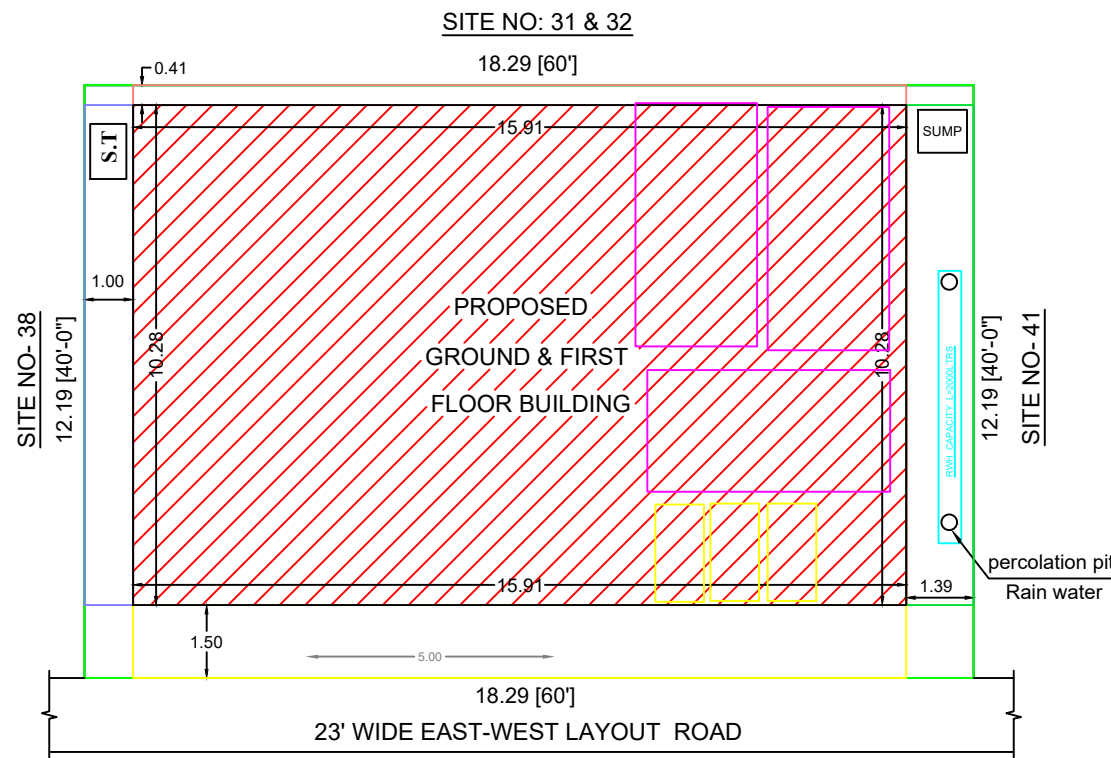
SITE PLAN
