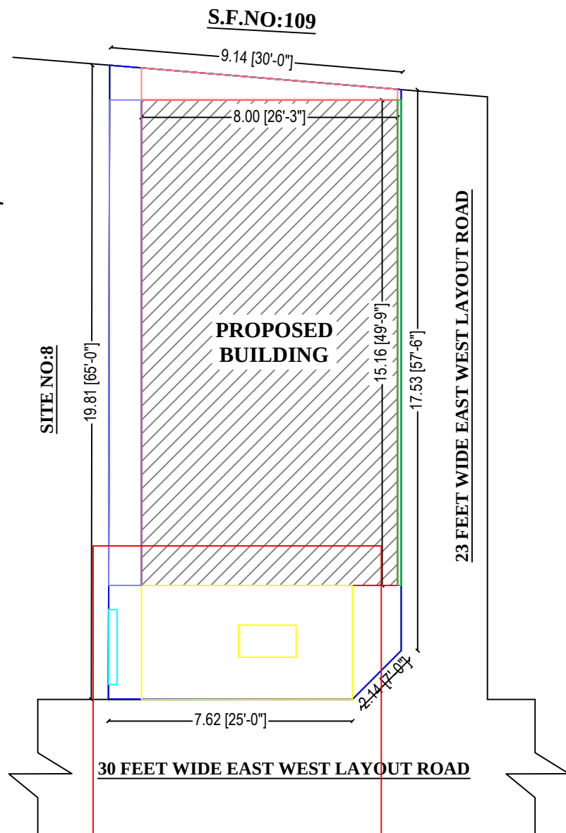
SITE PLAN
