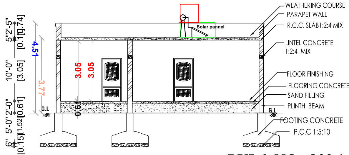
SECTION ON - A - A' PULA NO. 309 / 14 VACANT SITE & HOUSE .
