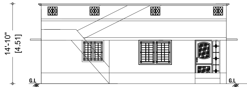
FRONT ELEVATION
