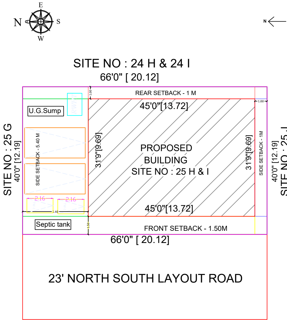
SITE PLAN
