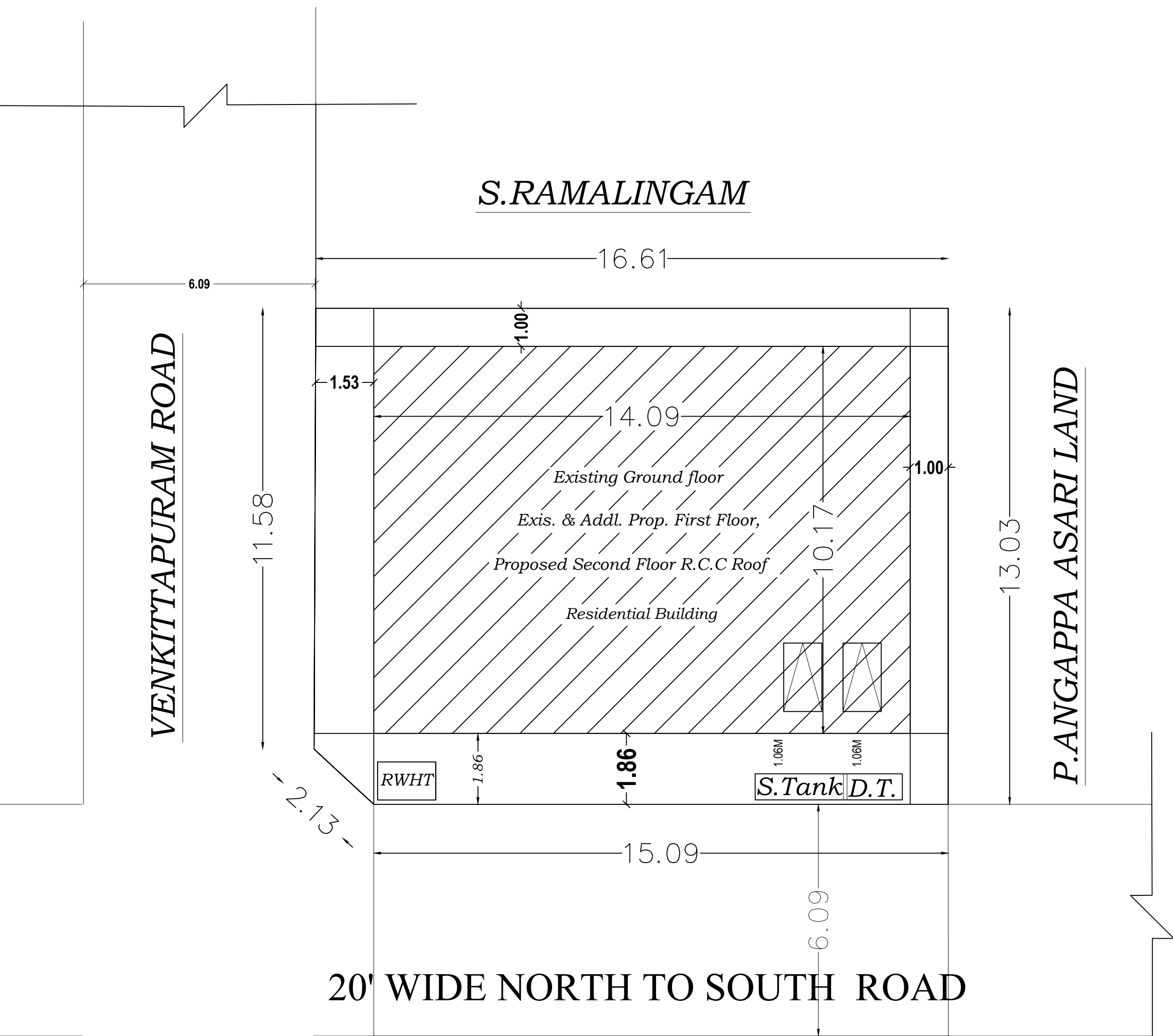
SITE PLAN
