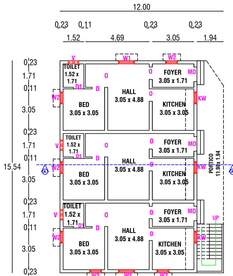
REVISED GROUND FLOOR PLAN
