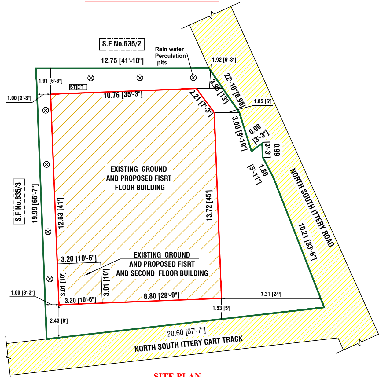
SITE PLAN
