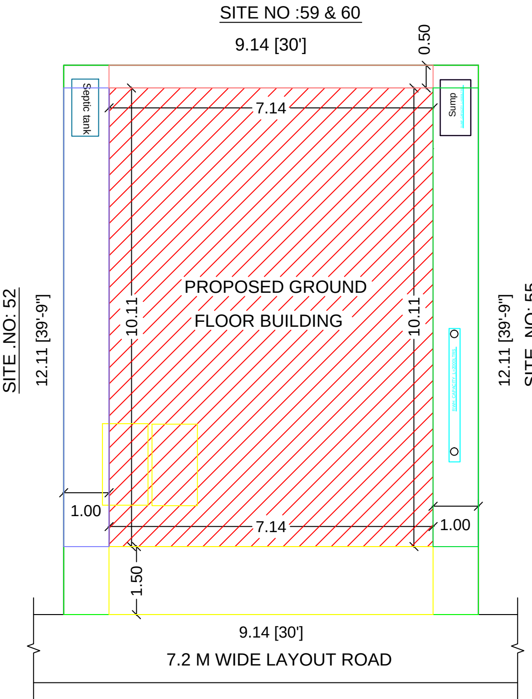
SITE PLAN
