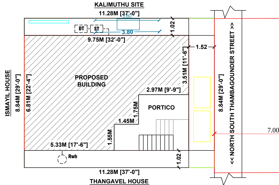
SITE PLAN
