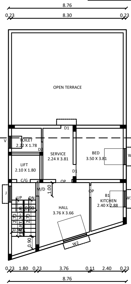
PRO. SECOND FLOOR (PT) PLAN
