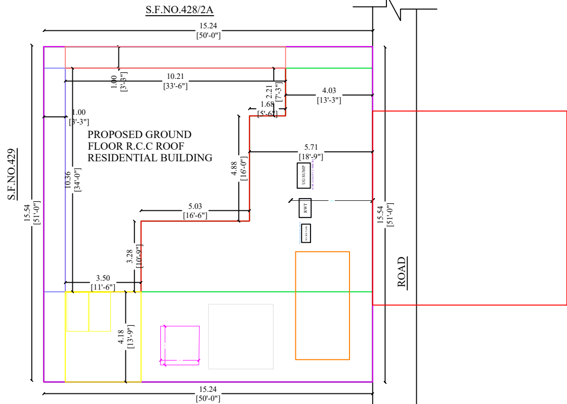
SITE PLAN OWNER'S REMAINING LAND
