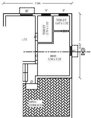
1. First Floor Plan
