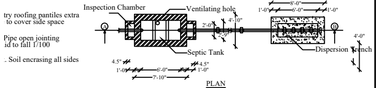
PLAN
