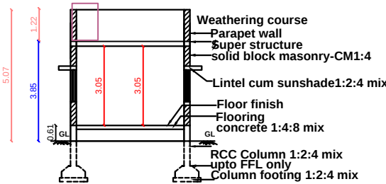
SECTION ELEVATION
