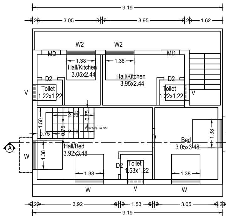
Plan Scale 1:100 Pro. First floor
