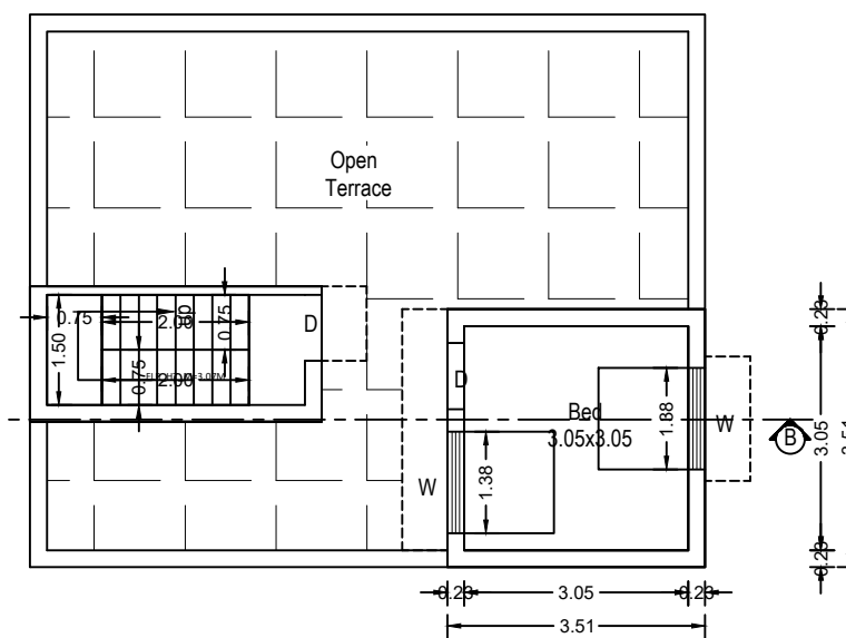
Plan Scale 1:100 Pro. Second floor
