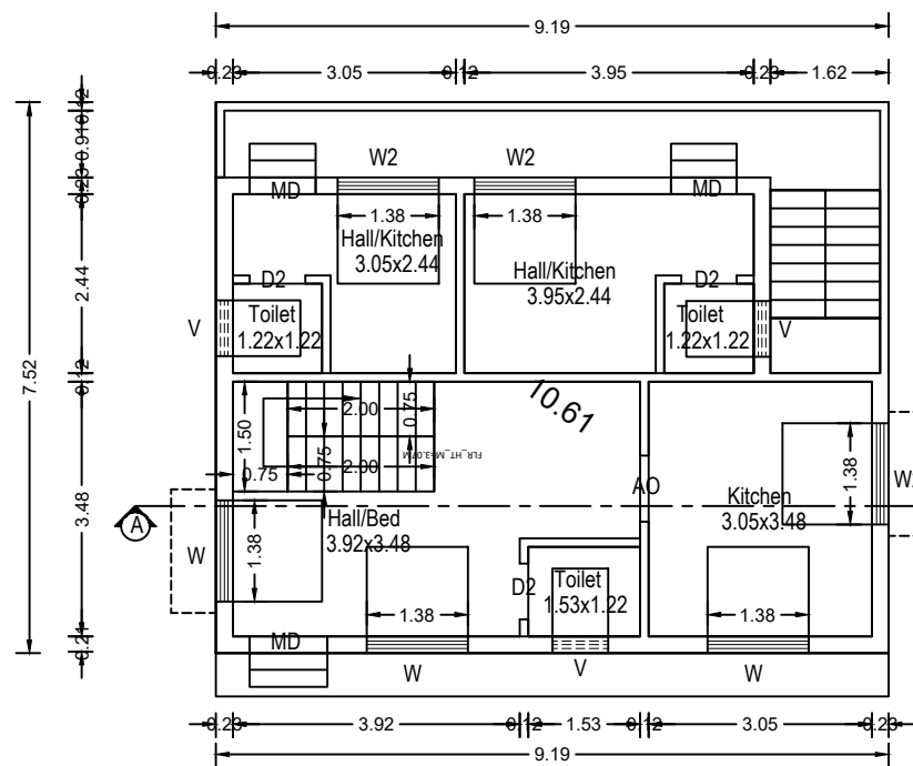
Plan Scale 1:100 Exg. Ground floor
