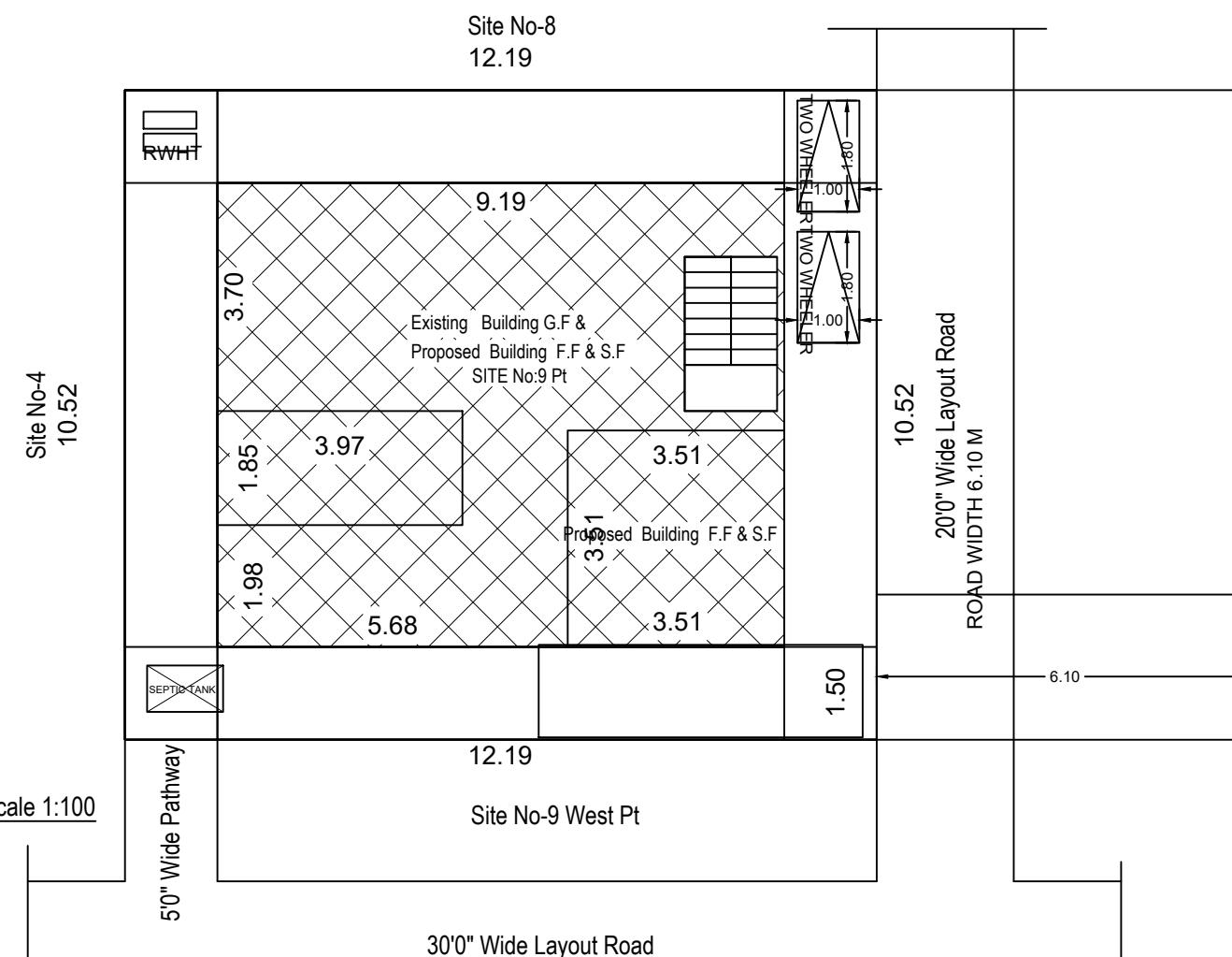
Plan Scale 1:100 Pro. Second floor
