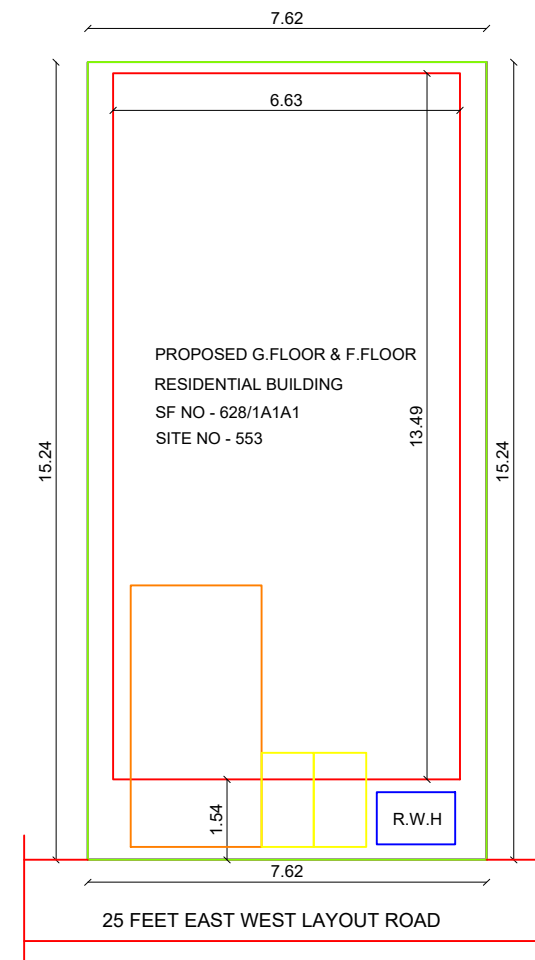
SITE PLAN
