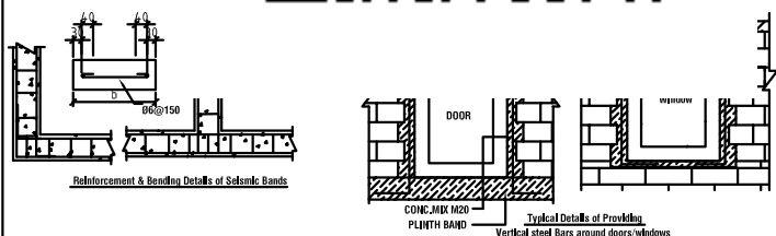
Essential Internal Elements in Buildings for Earthquake safety
