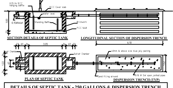
DETAILS OF SEPTIC TANK - 250 GALLONS & DISPERSION TRENCH
