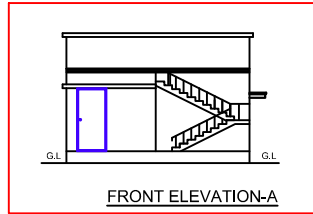
FRONT ELEVATION-A
