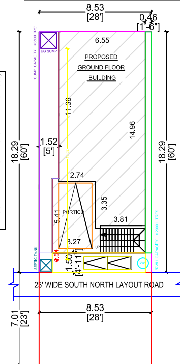
SITE PLAN
