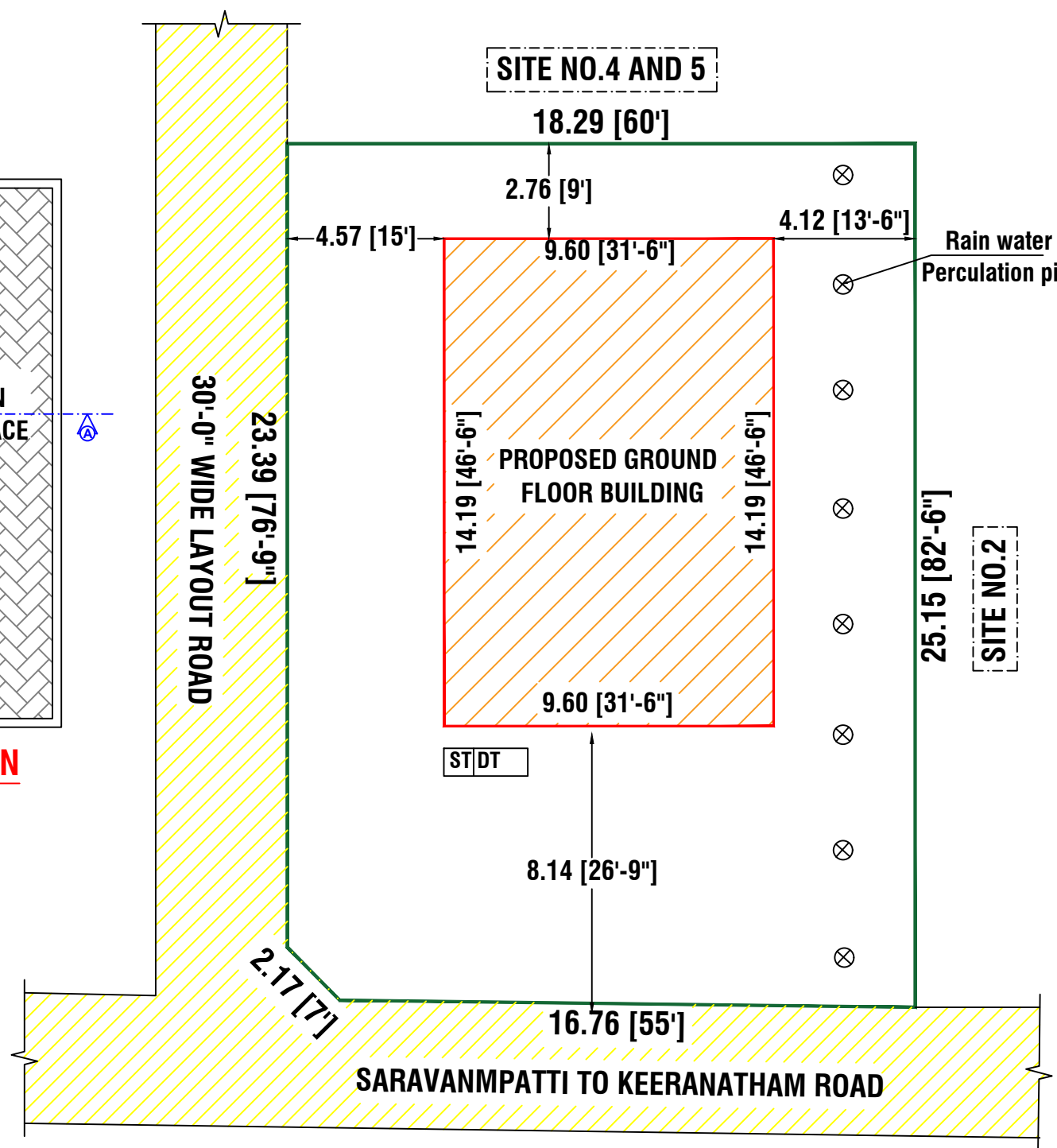
SITE PLAN
