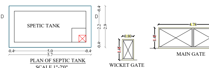
WICKET GATE
