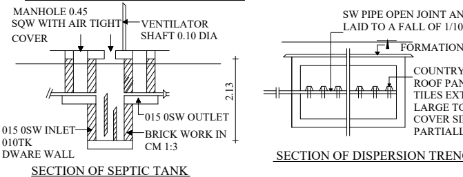
SECTION OF SEPTIC TANK
