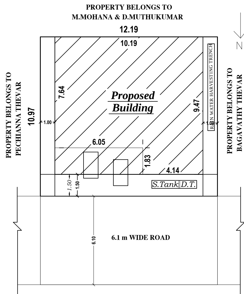
SITE PLAN
