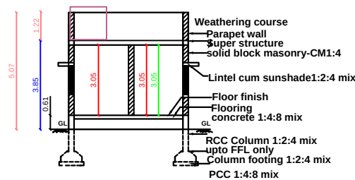
SECTION ELEVATION
