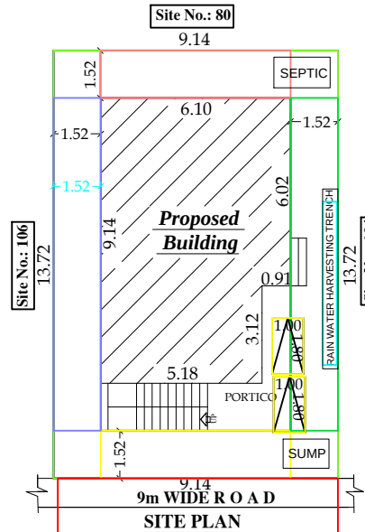
SITE PLAN
