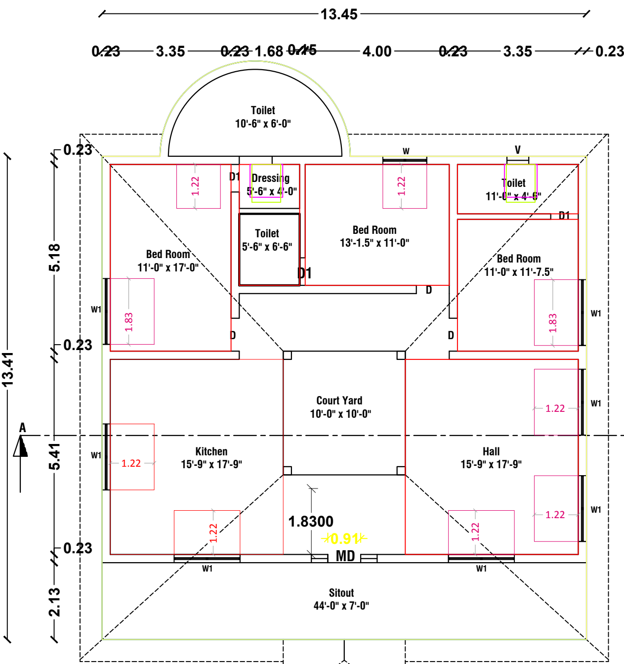
FLOOR PLAN
